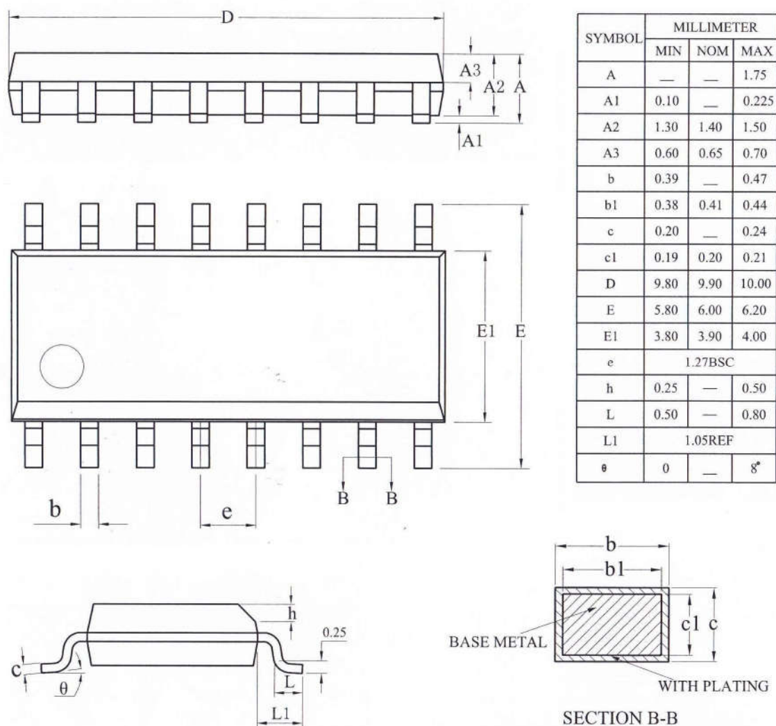
Figure 3-1. AC1042A_SOP16 Package
