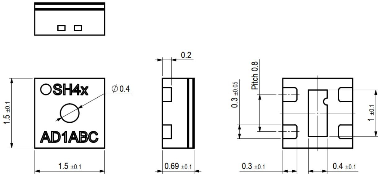
Figure 16. Dimensional drawing of SHT4x with filter membrane including package tolerances (units mm)
