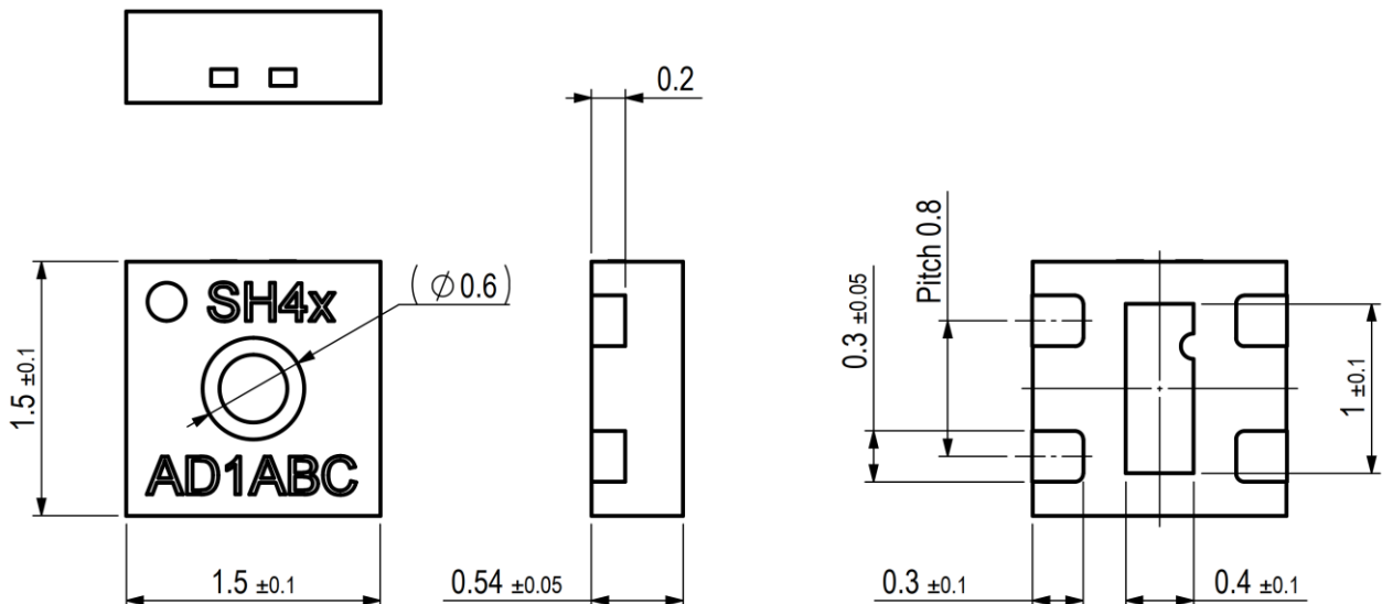
Figure 15. Dimensional drawing of SHT4x including package tolerances (units mm).
