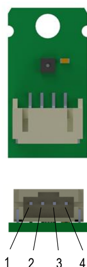
Figure 4. Connector pin assignment of the SCC30-DB module.
