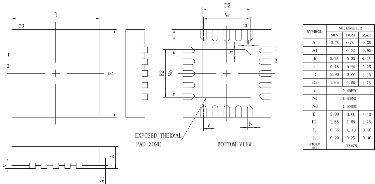
Figure 3-1 AC7003D Package
