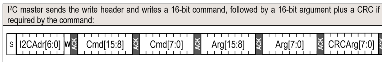
Figure 2: I 2 C sequence to send a command with an argument to the sensor.
