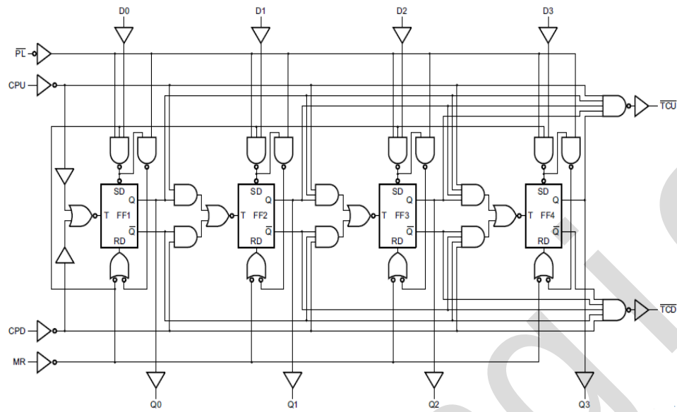
Figure 4. Logic diagram
