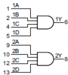
Figure 1. Logic symbol
