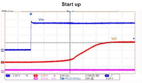
V_{IN} = 7V , C_{IN} = 1\mu F , C_{OUT} = 1\mu F , Load = NA
