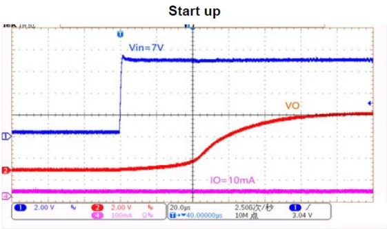
V_{IN} = 7V , C_{IN} = 1\mu F , C_{OUT} = 1\mu F , Load =10mA
