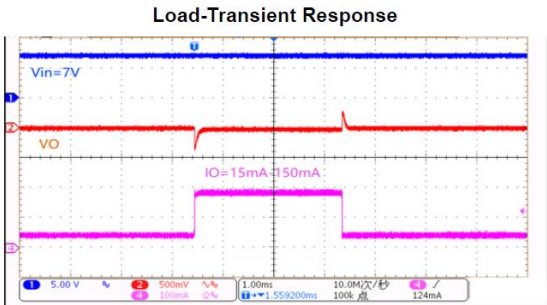
V_{IN} = 7V , C_{IN} = 1\mu F , C_{OUT} = 1\mu F
