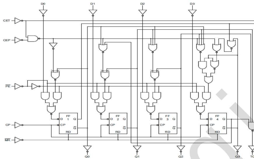
Figure 4. Logic diagram
