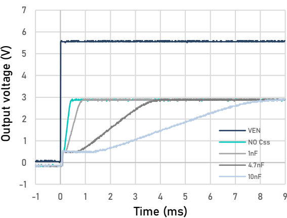
Figure 52. Typical soft start behavior, Different C SS values
