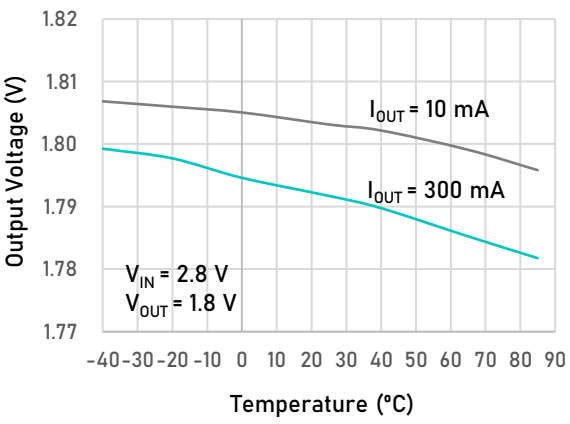
Output Voltage vs. Temperature V_{OUT} = 1.8\text{ V DFN2}\times 2-6
