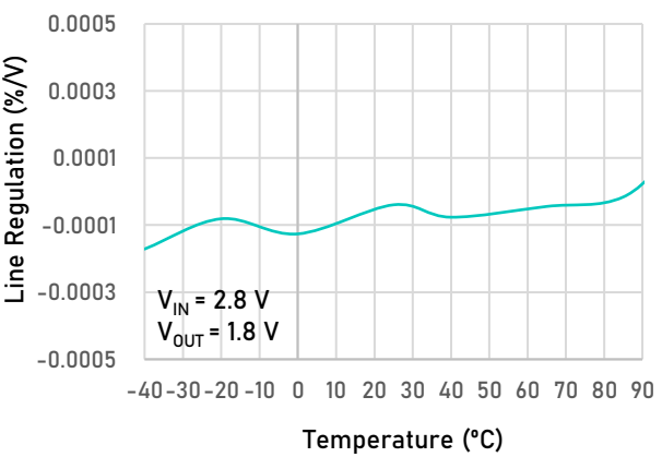
Line Regulation vs. Temperature V_{OUT} = 1.8\text{ V DFN2}\times 2-6
