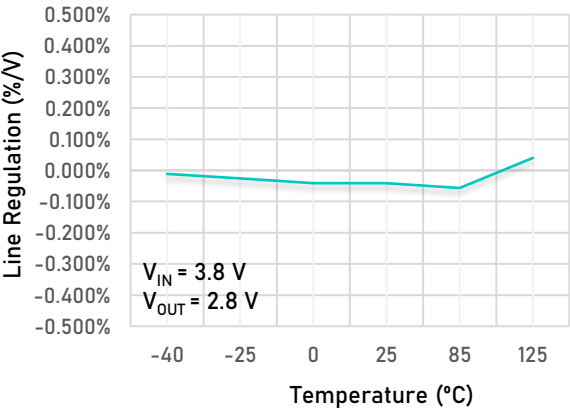
Line Regulation vs. Temperature V_{OUT} = 2.8\text{ V DFN1}\times 1-4
