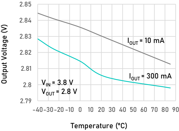
Output Voltage vs. Temperature V_{OUT} = 2.8\text{ V DFN1}\times 1-4
