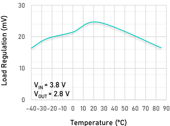
Load Regulation vs. Temperature V_{OUT} = 2.8\text{ V DFN1}\times 1-4
