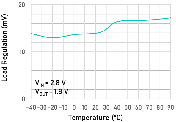
Load Regulation vs. Temperature V_{OUT} = 1.8\text{ V DFN2}\times 2-6
