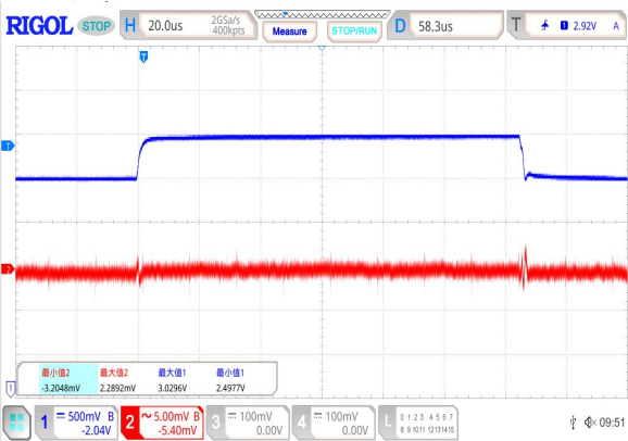
Time (20μs/div)
