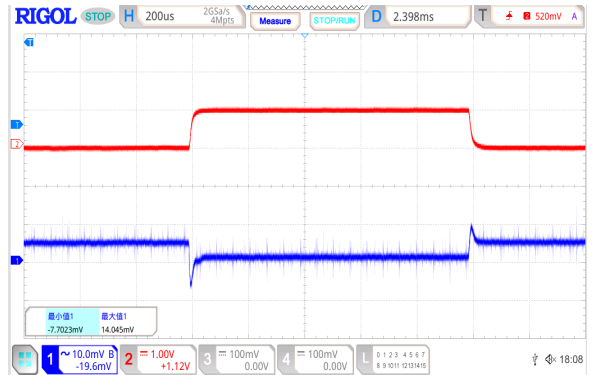
Figure 44. Load Transient Response, I_{LOAD} = 100\text{ mA} to 1.6\text{ A} , 1.2\text{ V} Adjustable version & V_{OUT} = 5\text{ V} , V_{IN} = 5.5\text{ V} , CH1 = V_{OUT} , CH2 = I_{LOAD}
