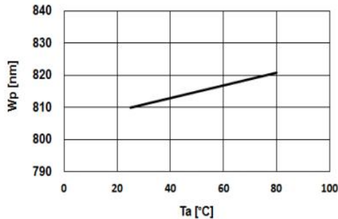
Fig.5 – Peak Wavelength (@500mA) vs. Ambient Temperature
