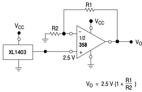
Figure 10. Voltage Reference
