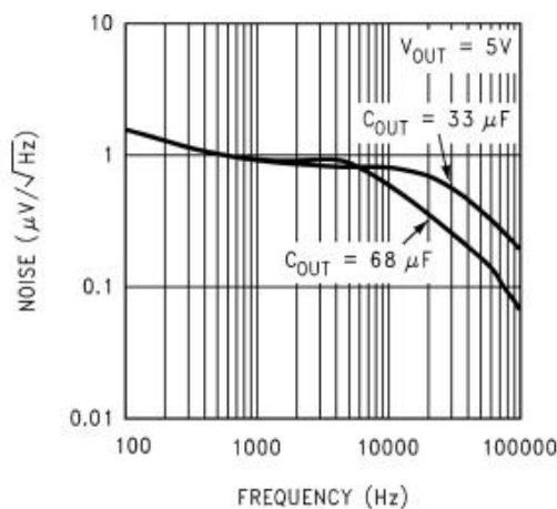
Output Noise Density, V_{OUT} = 5V
