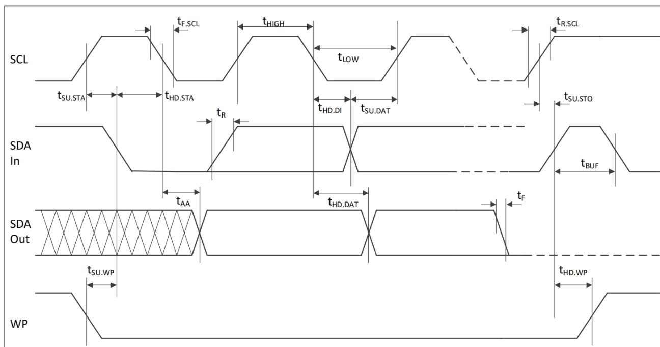
Figure 18 Bus Timing
