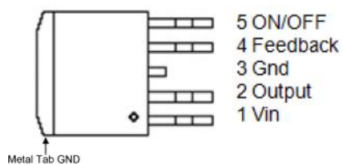
TO -252-4
