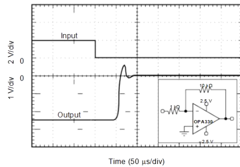
Figure 12. 负过压恢复
