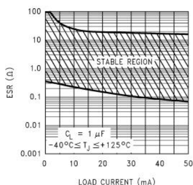
FIGURE 1. 1 \mu\text{F} ESR Range
