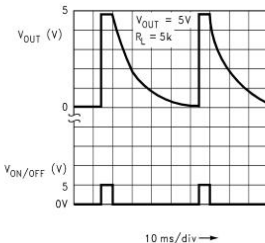
Turn-Off Waveform
