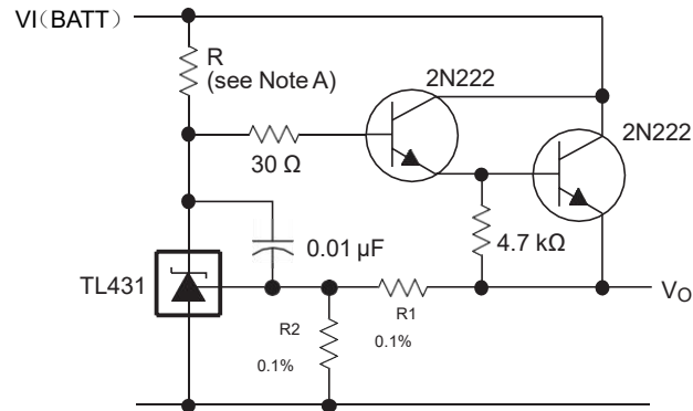
Figure 29. Precision High-Current Series Regulator
