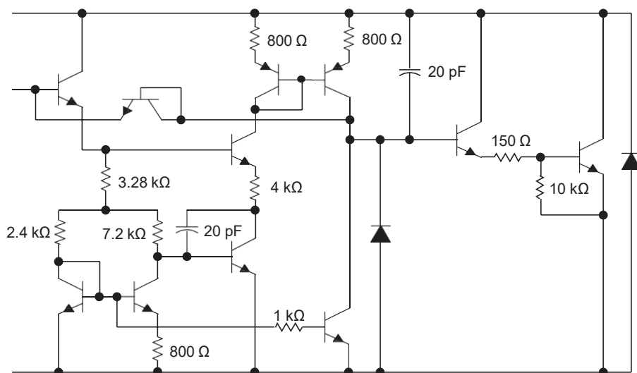
Figure 24. Detailed Schematic
