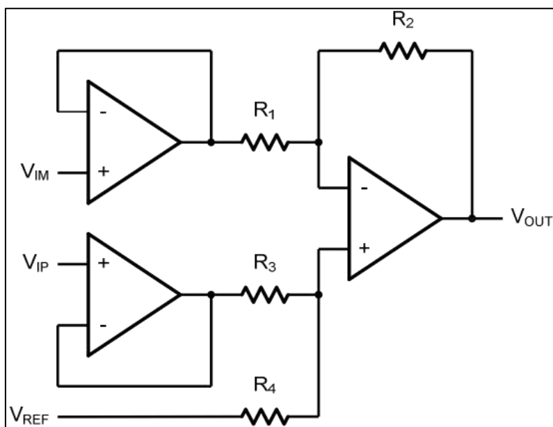
Figure 6. Instrument Amplifier
