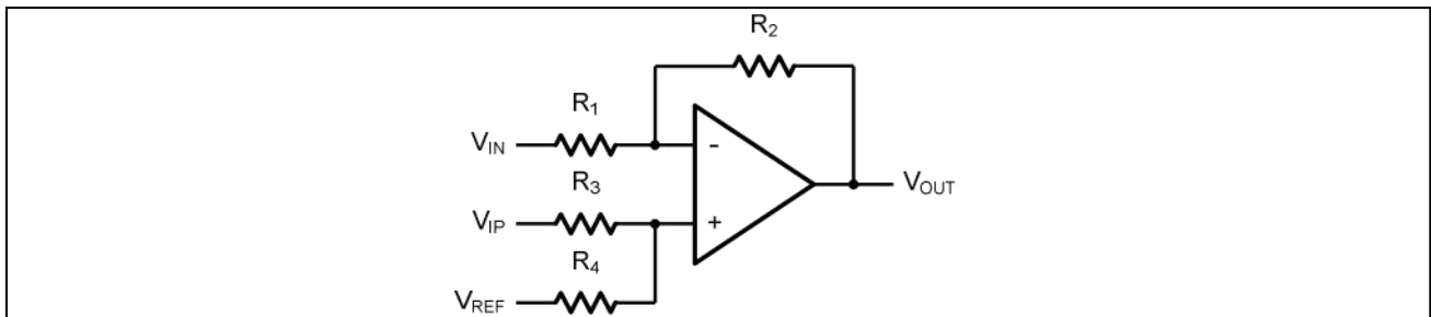
Figure 4. Differential Amplifier
