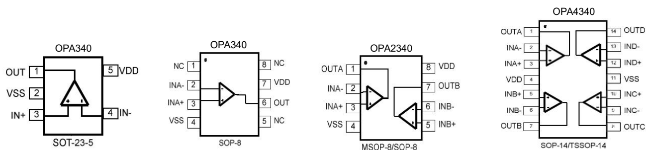
Figure 1. Pin Assignment Diagram
