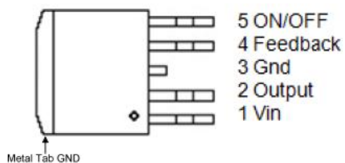
TO -252-4
