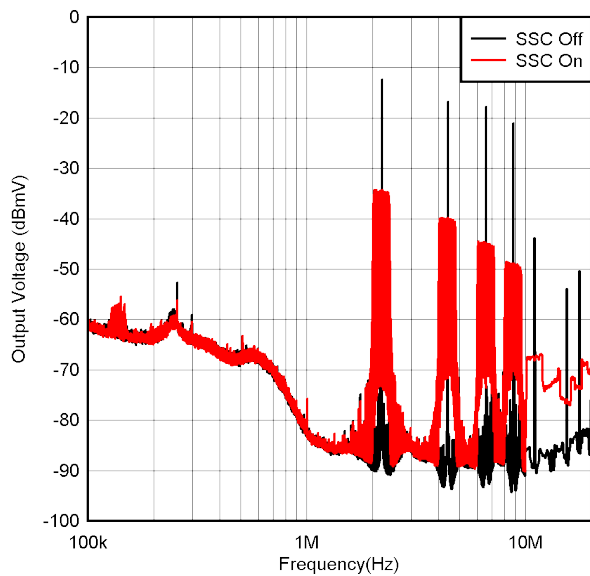
V_{OUT} = 0.75 \text{ V} I_{OUT} = 11.5 \text{ A} Figure 10-18. Spread Spectrum Operation
