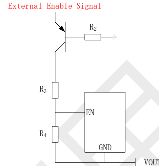
Figure 3. Enable Control Circuit for Negative Output
