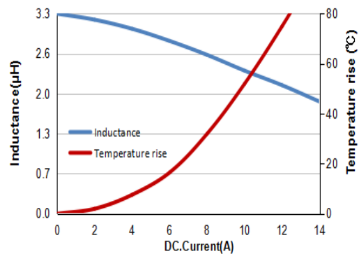
FSA0650-3R3MT
