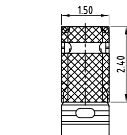
RECOMMENDED PCB LAYOUT TOLERANCE:±0.05MM (FOR REFERENCE ONLY)
