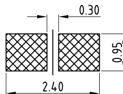
METAL MASK T=0.08 TOLERANCE:±0.05MM (FOR REFERENCE ONLY)
