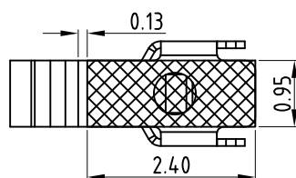
RECOMMENDED PCB LAYOUT TOLERANCE:±0.05MM (FOR REFERENCE ONLY)
