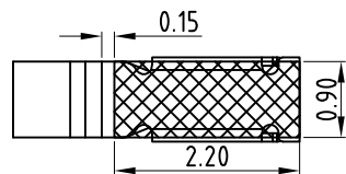
RECOMMENDED PCB LAYOUT TOLERANCE: ±0.05MM (FOR REFERENCE ONLY)
