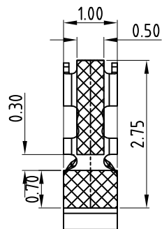
RECOMMENDED PCB LAYOUT TOLERANCE:±0.05MM (FOR REFERENCE ONLY)
