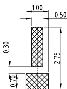
METAL MASK T=0.08 TOLERANCE:±0.05MM (FOR REFERENCE ONLY)
