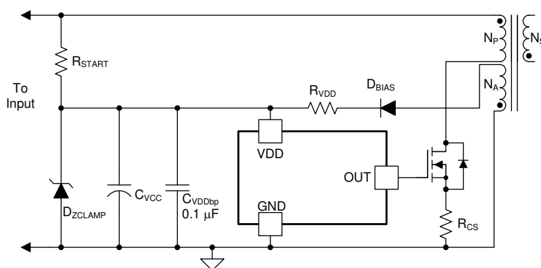
Figure 8-1. VDD Protection
