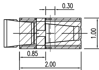
RECOMMENDED PCB LAYOUT TOLERANCE±0.05(焊盘推荐图)
