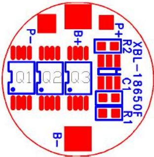
BOTTOM SILKSCREEN
