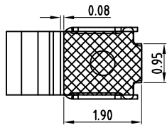
RECOMMENDED PCB LAYOUT TOLERANCE: ±0.05MM (FOR REFERENCE ONLY)
