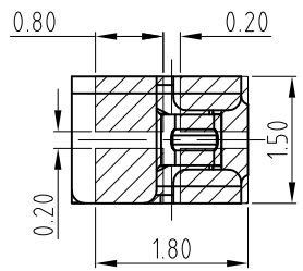
RECOMMENDED PCB LAYOUT TOLERANCE±0.05(焊盘推荐图)
