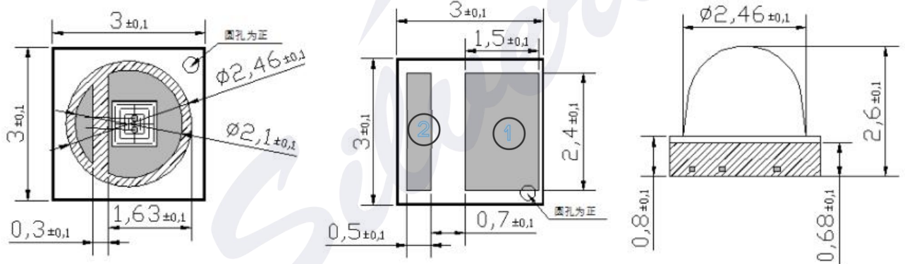
焊点结构 Pad Configuration:
