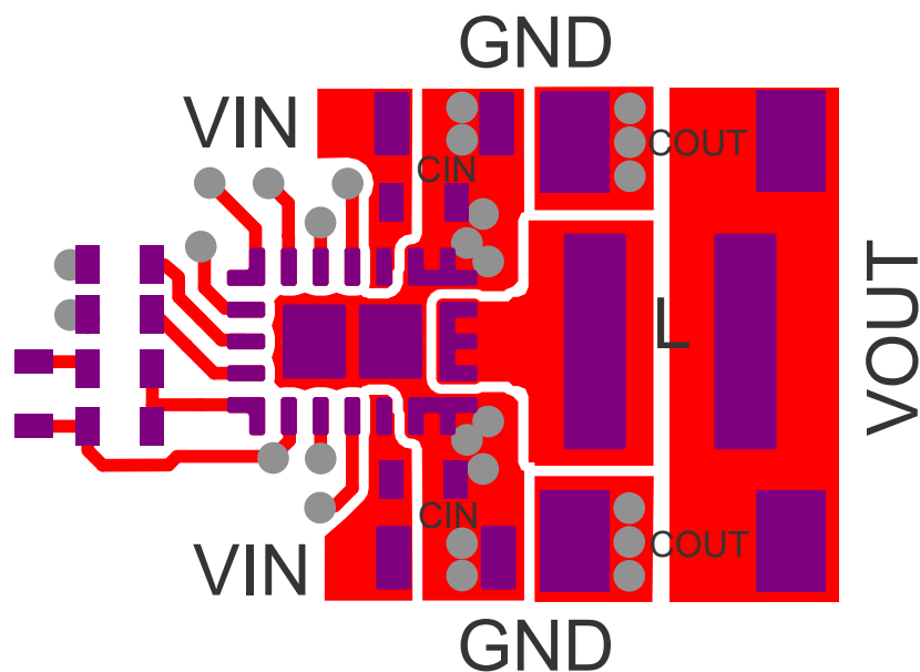
Figure 10-24. Layout Example
