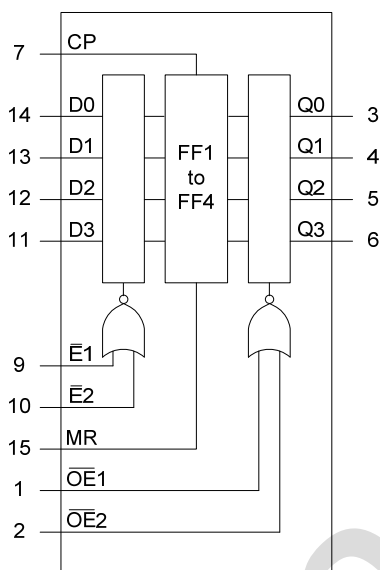
Figure 1. Functional diagram
