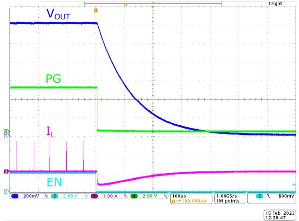
Figure 9-9. Shutdown With No Load (TPS62A06)
