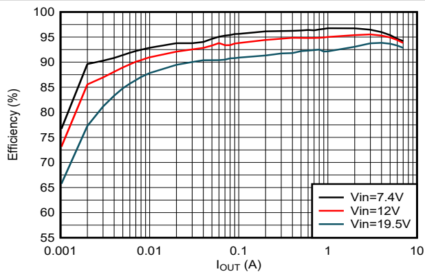
Figure 8-2. Efficiency, PSM Mode
