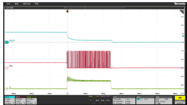
Figure 8-17. Normal Operation to Output Hard Short
