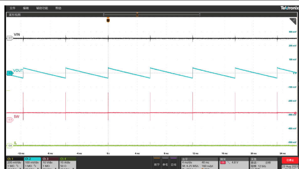
Figure 8-12. Output Voltage Ripple, Iout = 0 A, PSM Mode
