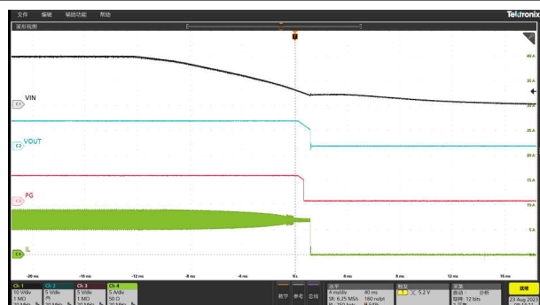
Figure 8-11. Shutdown Relative to Vin Falling, Iout = 7A
