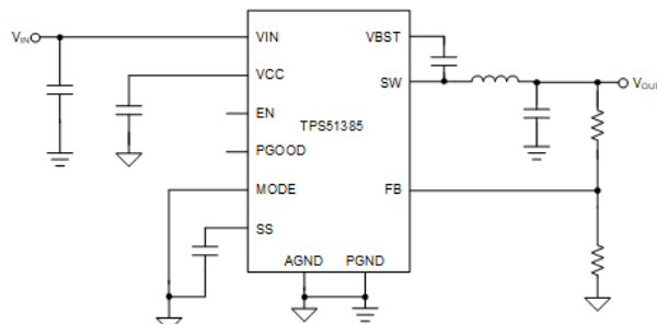
Typical Application
