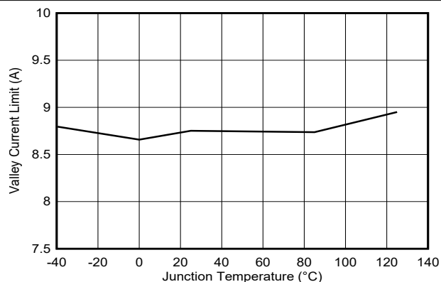
Figure 6-8. Valley Current Limit vs Temperature
