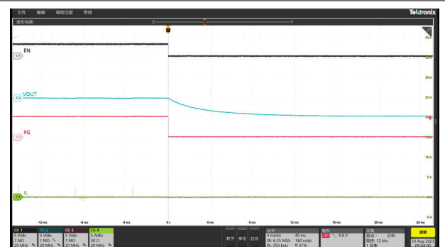
Figure 8-7. Shutdown Relative to EN Falling, Iout = 0A, PSM Mode
