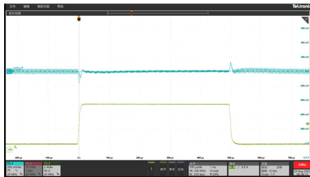
Figure 8-16. Transient Response, 0.7 A to 6.3 A with 2.5 A/us SR
