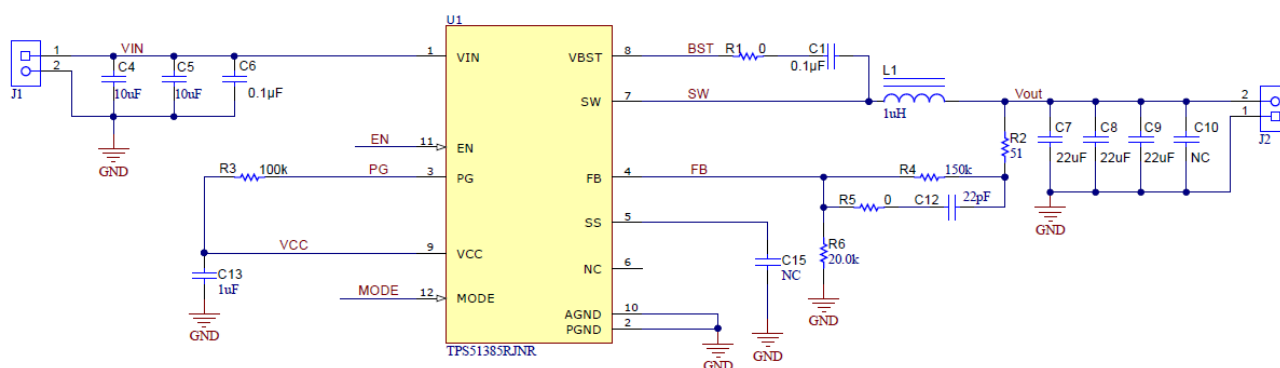
Figure 8-1. Application Schematic
