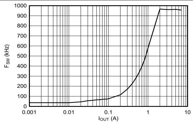
Figure 8-5. Switching Frequency, OOA Mode
