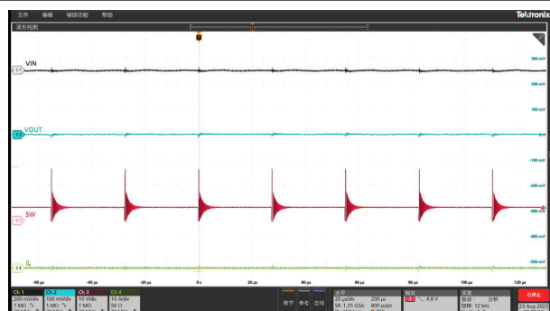
Figure 8-13. Output Voltage Ripple, Iout = 0 A, OOA Mode
