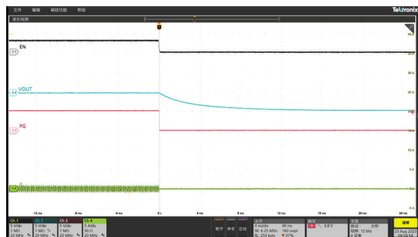
Figure 8-9. Shutdown Relative to EN Falling, Iout = 0A, OOA Mode
