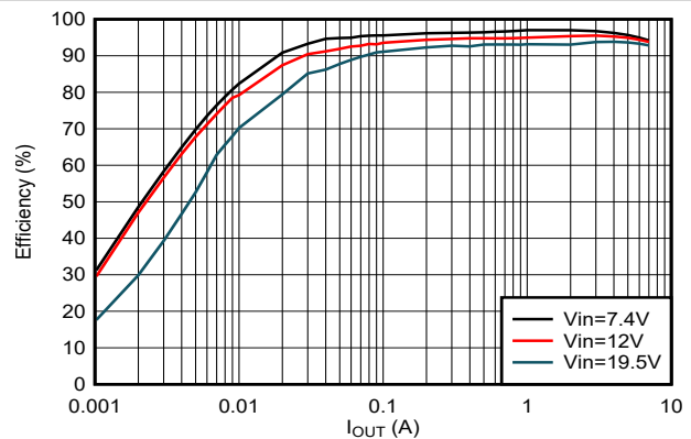
Figure 8-3. Efficiency, OOA Mode
