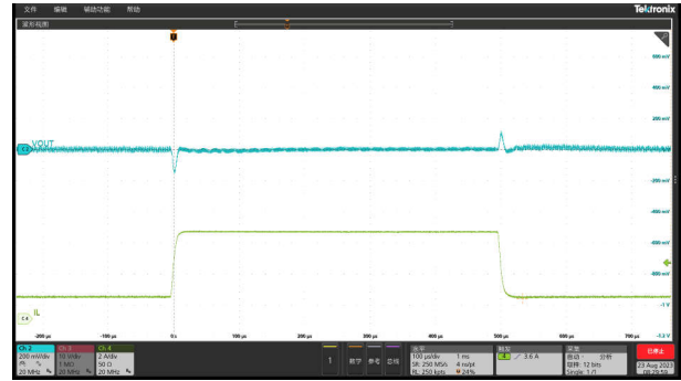
Figure 8-15. Transient Response, 1.4 A to 5.6 A with 2.5 A/us SR
