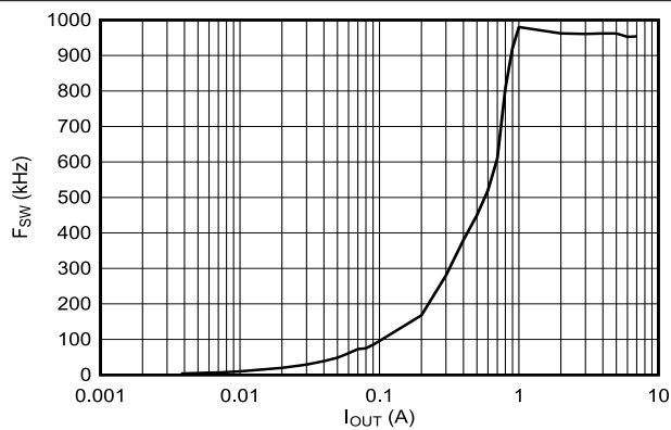
Figure 8-4. Switching Frequency, PSM Mode
