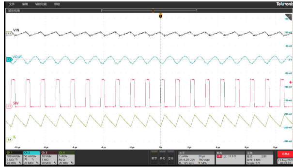
Figure 8-14. Output Voltage Ripple, Iout = 7 A
