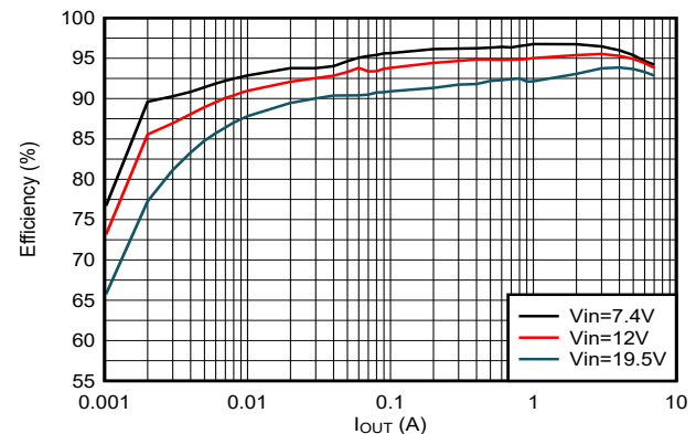
Efficiency Curve, V_{OUT} = 5.1 V, PSM Mode
