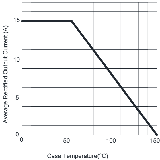
FIG1:Io-Tc Curve
