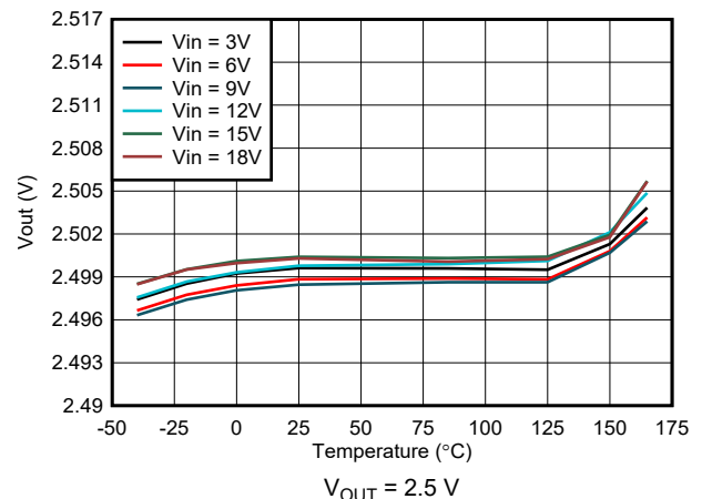
Figure 7-6. Output Voltage Accuracy - VSET Selected
