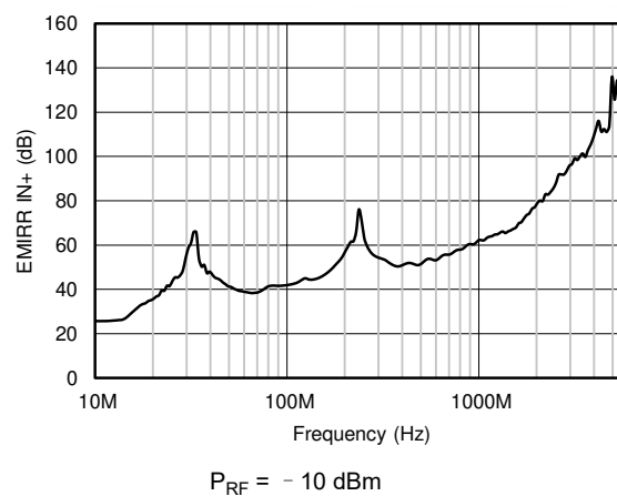
图 6-38. EMIRR vs Frequency
