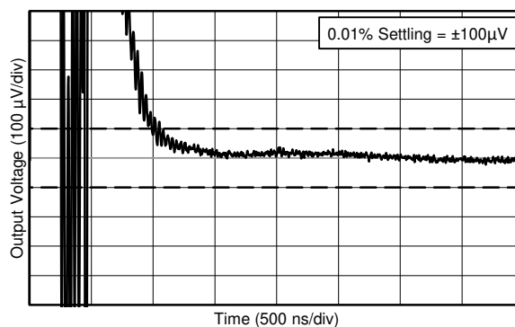
图 6-32. Large-Signal Step Response (4-V Step)
