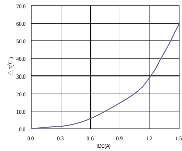
CM32251R0□S□
