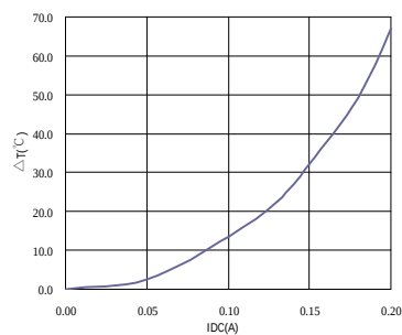
CM3225121□S□
