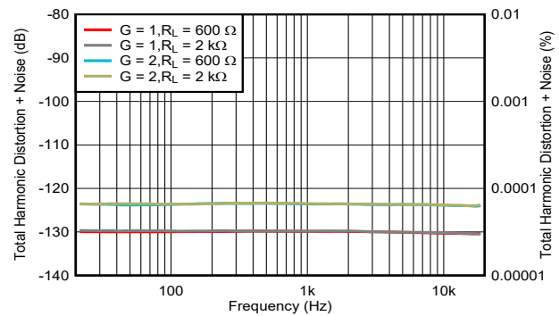
Figure 5-32. THD+N vs Frequency
