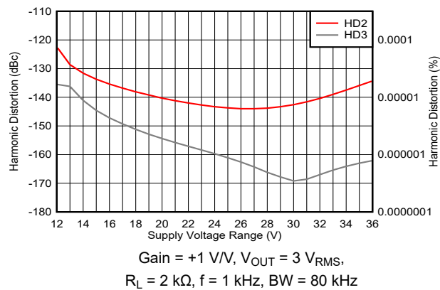
Figure 5-41. Distortion Harmonics vs Supply Voltage
