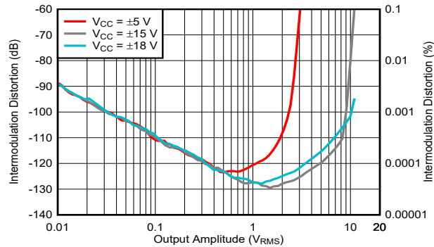
Figure 5-37. Intermodulation Distortion vs Amplitude
