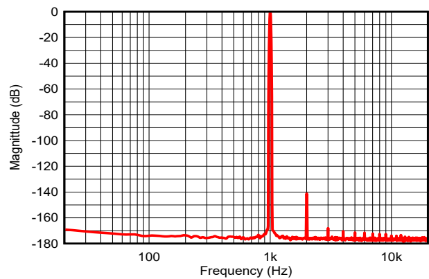
Figure 5-42. 1-kHz Output Spectrum
