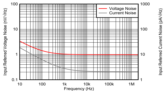
Voltage and Current Noise vs Frequency
