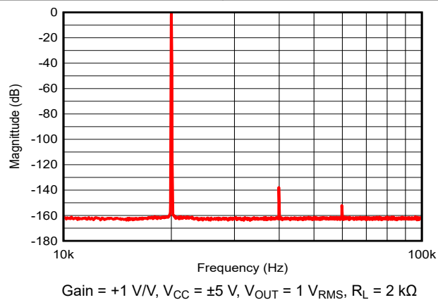
Figure 5-43. 20-kHz Output Spectrum
