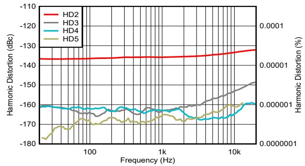
Figure 5-38. Distortion Harmonics vs Frequency
