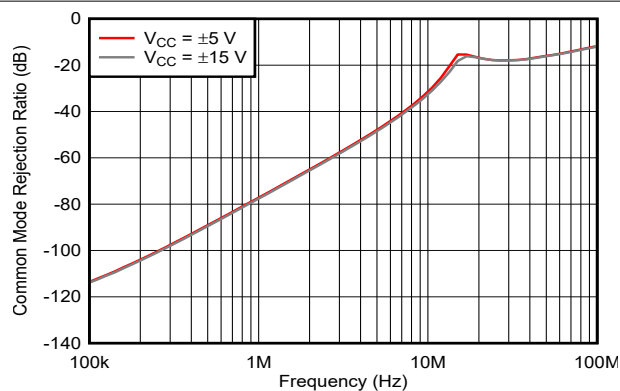
Figure 5-12. Common-mode Rejection Ratio vs Frequency
