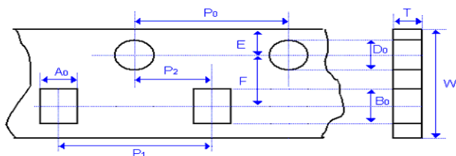
Fig. 9.1 The dimension of paper tape
