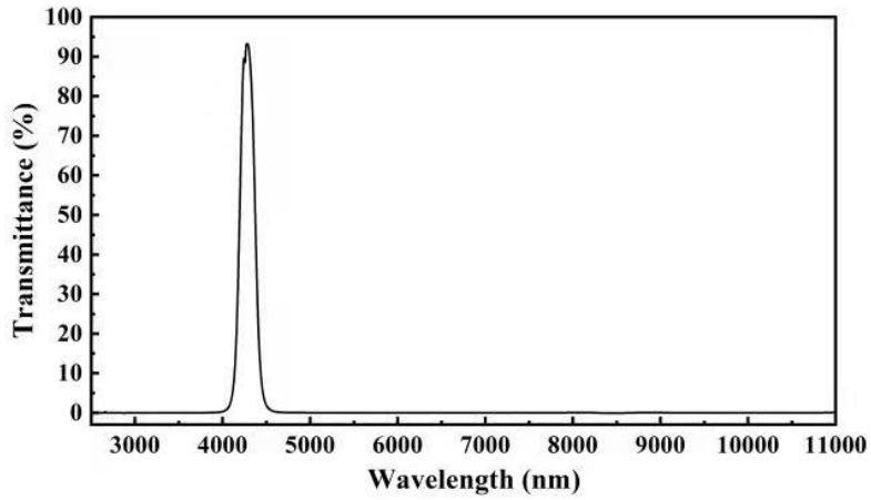
Transmittance of 4.26 μm Filter
