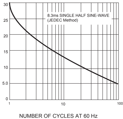
Fig. 3 Maximum Peak Forward Surger Current (per leg)
