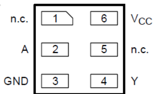
XSON6
