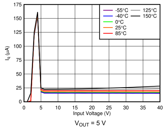
Figure 6-28. Quiescent Current ( I_Q ) vs V_{IN}
