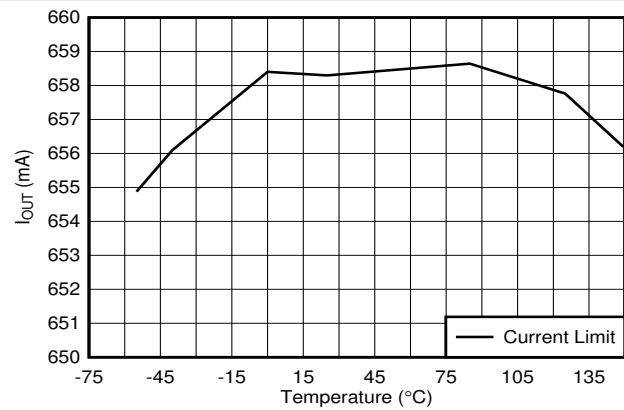
Figure 6-26. Output Current Limit vs Temperature
